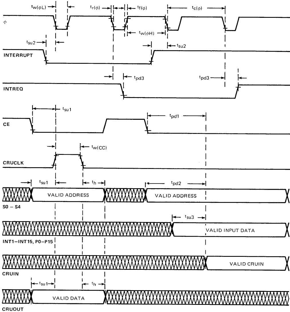
FIGURE 12—SWITCHING CHARACTERISTICS
