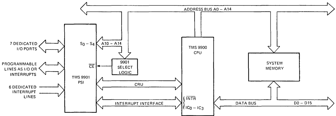
FIGURE 1— TYPICAL TMS 9901 PROGRAMMABLE SYSTEM INTERFACE (PSI) APPLICATION
