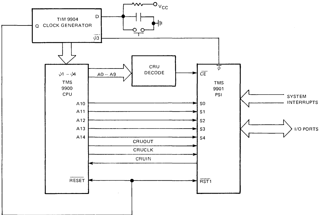
FIGURE 7—TMS 9900/TMS 9901 INTERFACE
